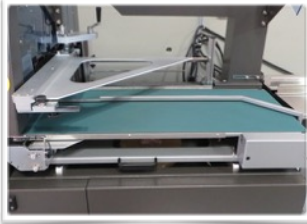
Adjustable inverting triangle for pkg height adjustment
