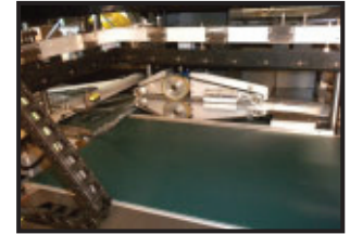
Vertical seal head with one piece seal knife and blade
