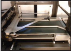
Motorized inverting triangle for pkg height adjustment
